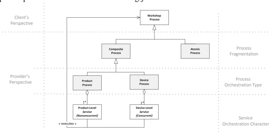
Fig. 2. Processes Types
