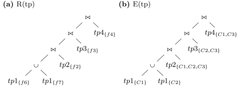
Fig. 4: Execution plan encoded in data structures R and E; multiple subsets represent union of different fragment (ex. {f 6 }, {f 7 }); elements of the subset represent alternative location of fragments (ex. {C 1 ,C 3 }); bold sources are the selected sources after set covering is used to reduce the sources
